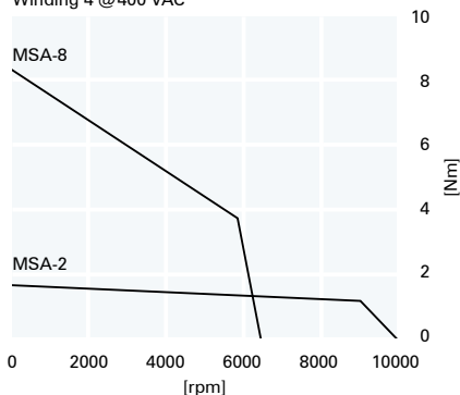
Winding 4 @ 400 VAC
