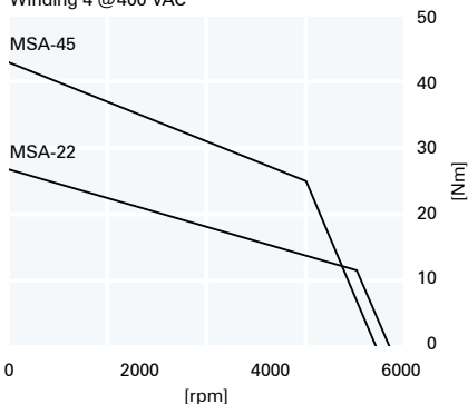
Winding 4 @ 400 VAC
